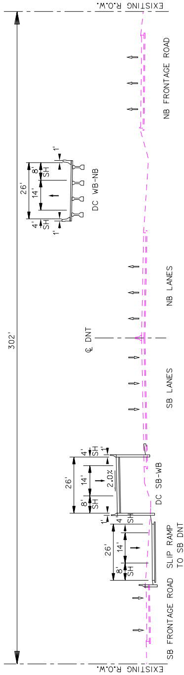
DNT PROPOSED TYPICAL SECTION
