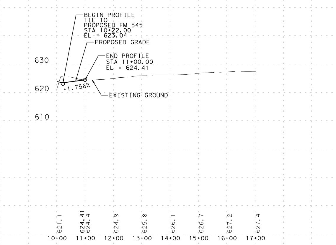
CR 575 PROFILE (ROLL 6 OF 8)
