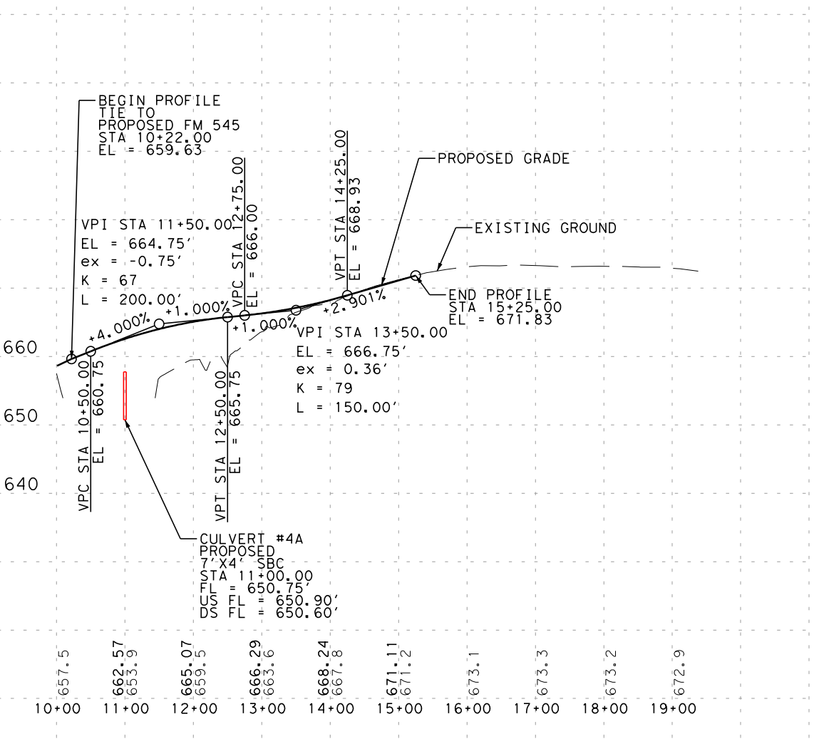
CR 415 PROFILE (ROLL 1 OF 8)
