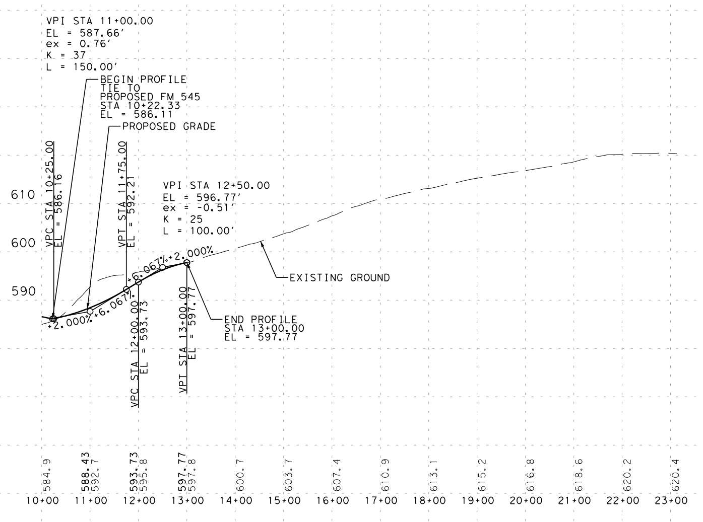
CR 472 PROFILE (ROLL 3 OF 8)
