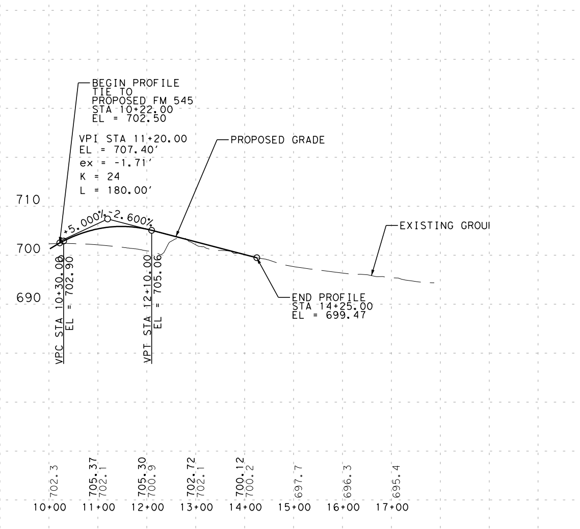
CR 416 PROFILE (ROLL 2 OF 8)
