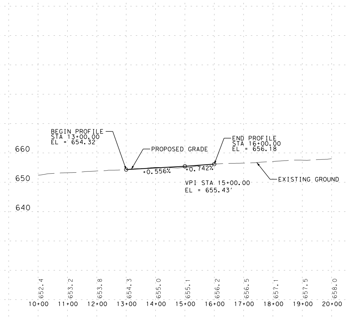
FM 2933 PROFILE (ROLL 1 OF 8)
