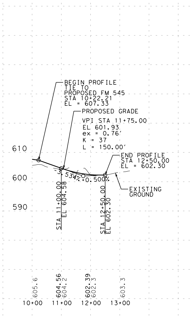
CR 1095 PROFILE (ROLL 3 OF 8)
