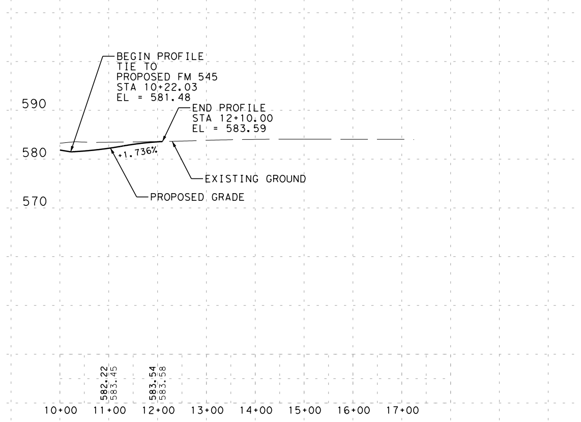
FM 1377 PROFILE (ROLL 6 OF 8)
