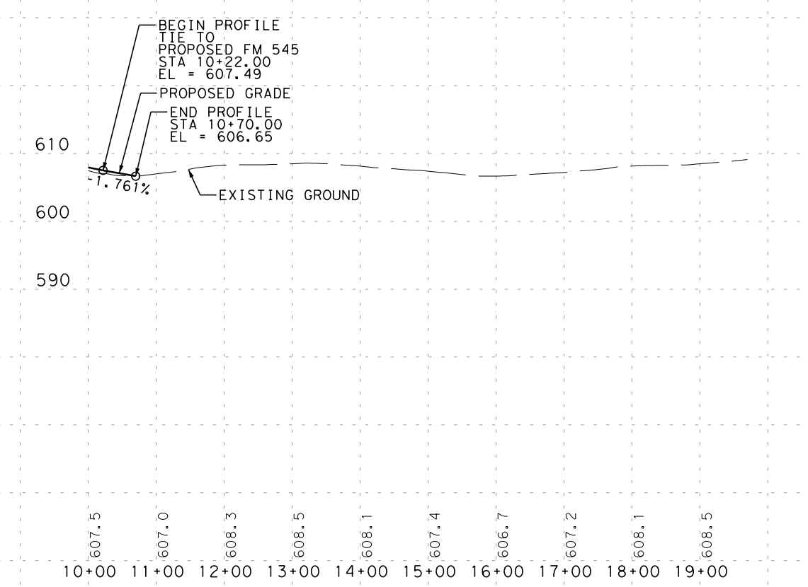
CR 475 PROFILE (ROLL 4 OF 8)
