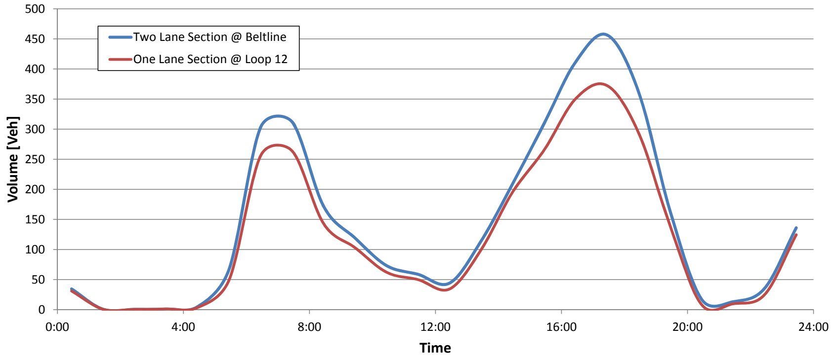
I-30W HOV Lanes Average Weekday Hourly Volume (Period 9/26/11 - 10/8/11)
