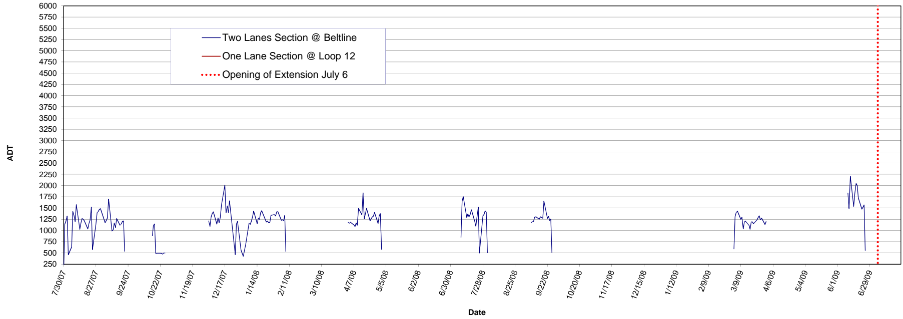
IH-30W Managed HOV ADT Before Opening of Extension, w/o Weekends & Holidays (Tube Counters)
