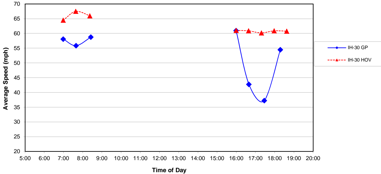
Average Speed Comparison IH-30W Main Lanes vs. Managed HOV Lanes, Sep 2011
