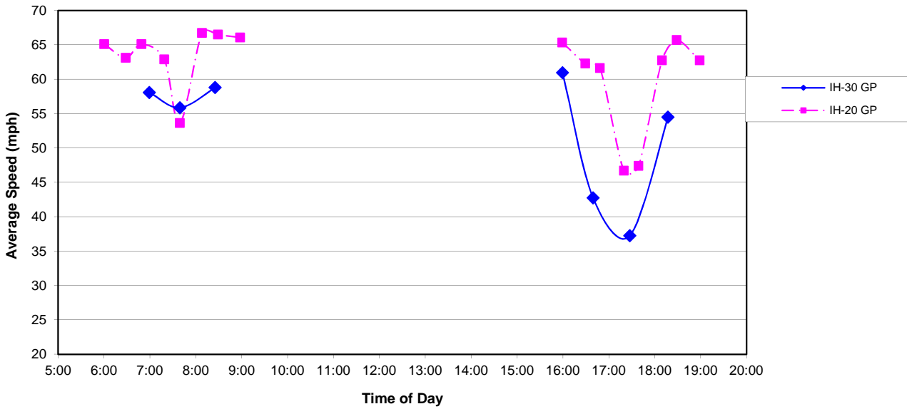
Average Speed Comparison IH-30W vs. IH-20 Main Lanes Sep 2011
