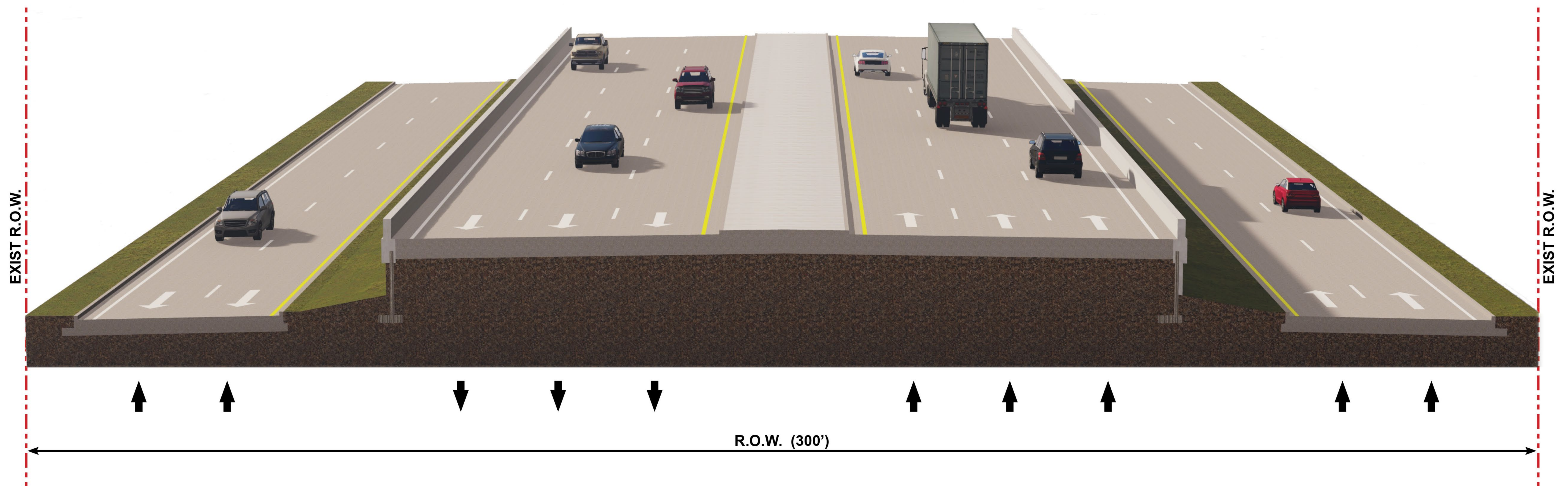
EXISTING TYPICAL SECTIONS (Mahard Parkway to Lovers Lane in Collin County)
