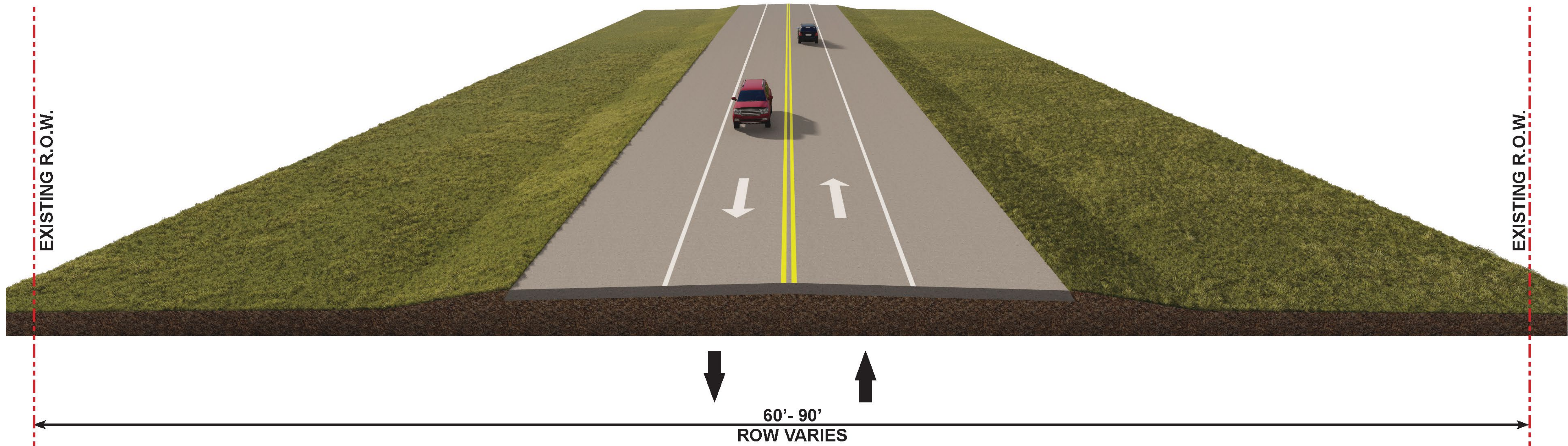
FM 1777 EXISTING TYPICAL SECTION From SH 66 to FM 6 in Collin County
