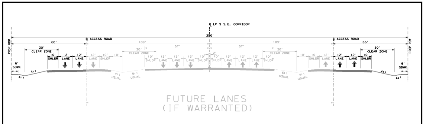
Figure 7-3: Corridor/Feasibility Study Typical Section
