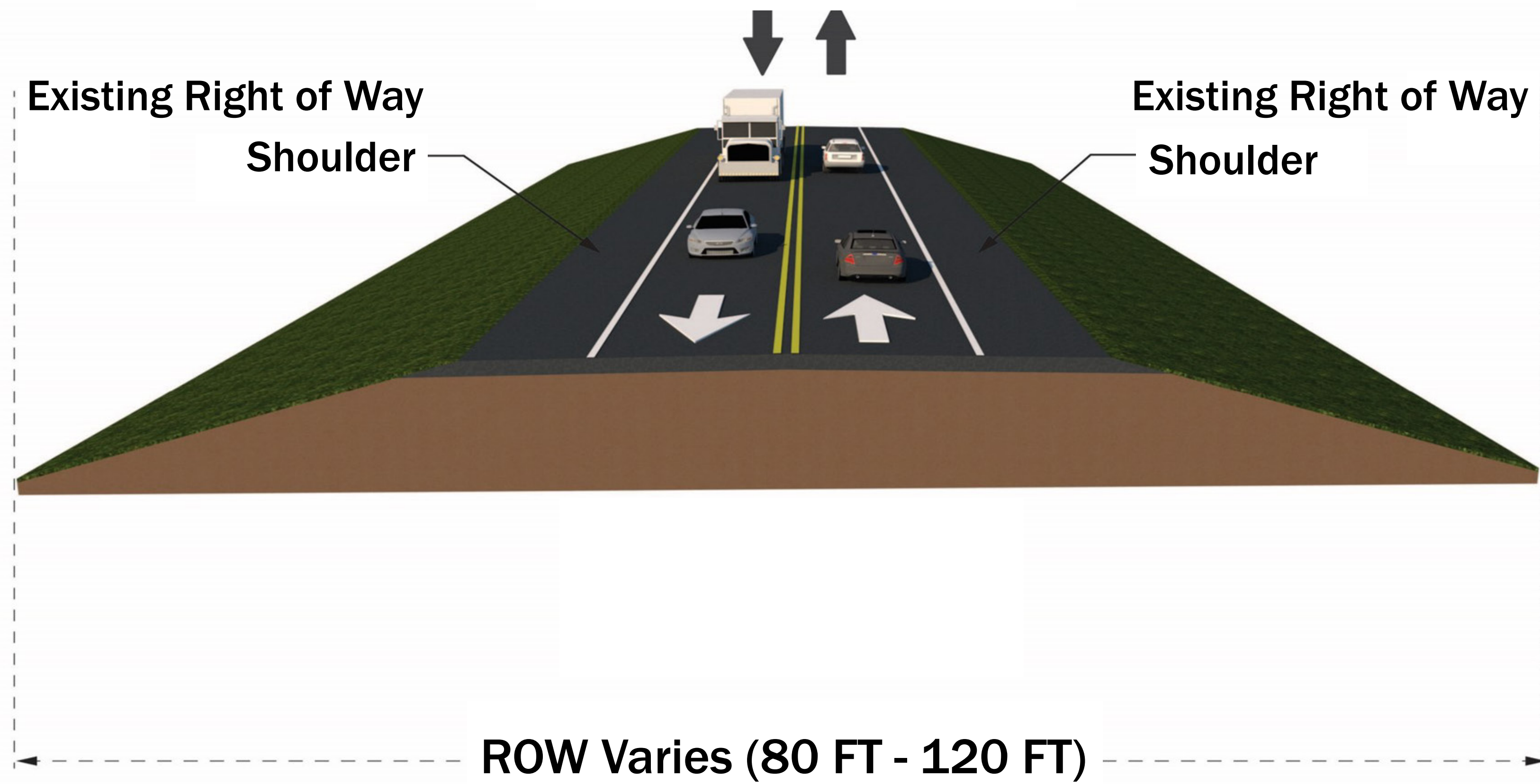
Existing FM 1385
