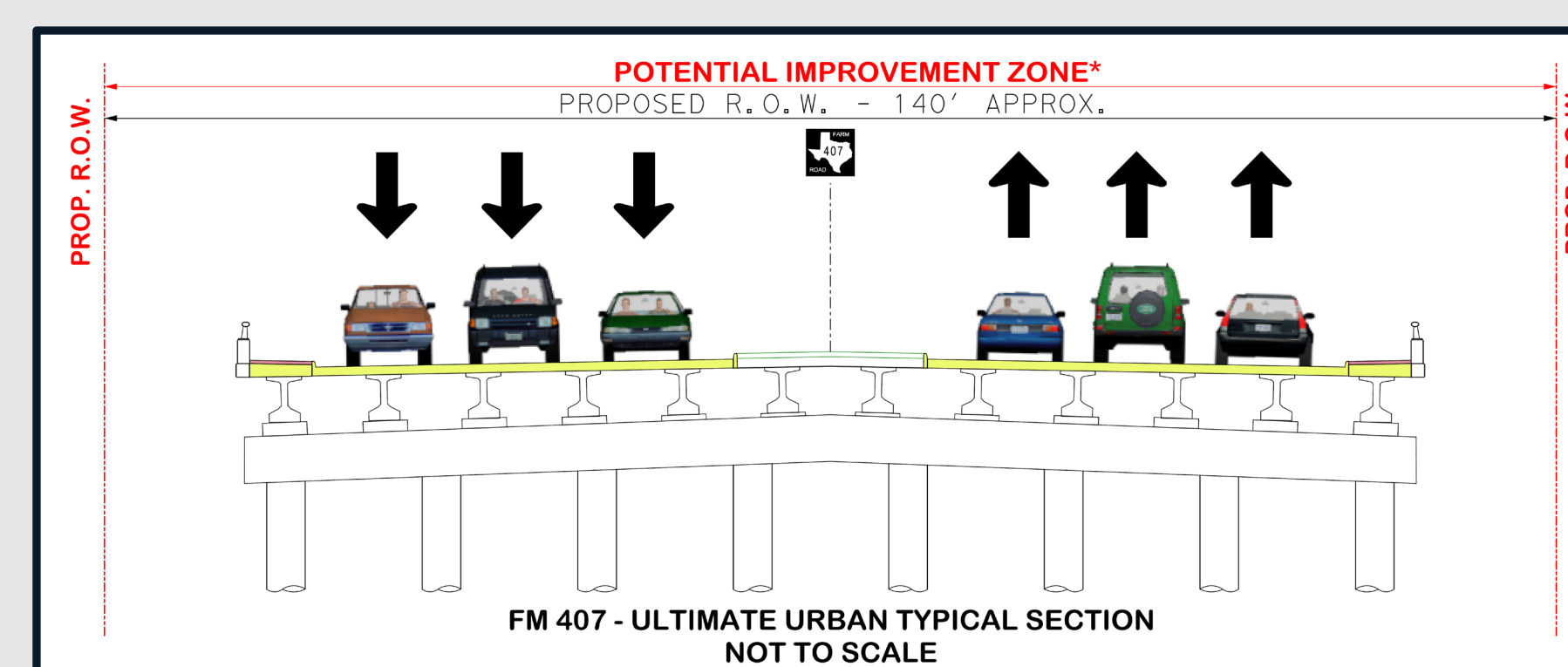
Typical Section A Concept
