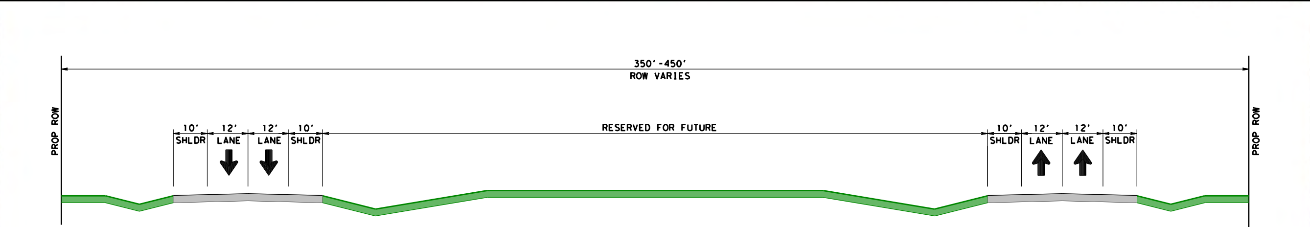
PROPOSED SECTION LOOP 9
