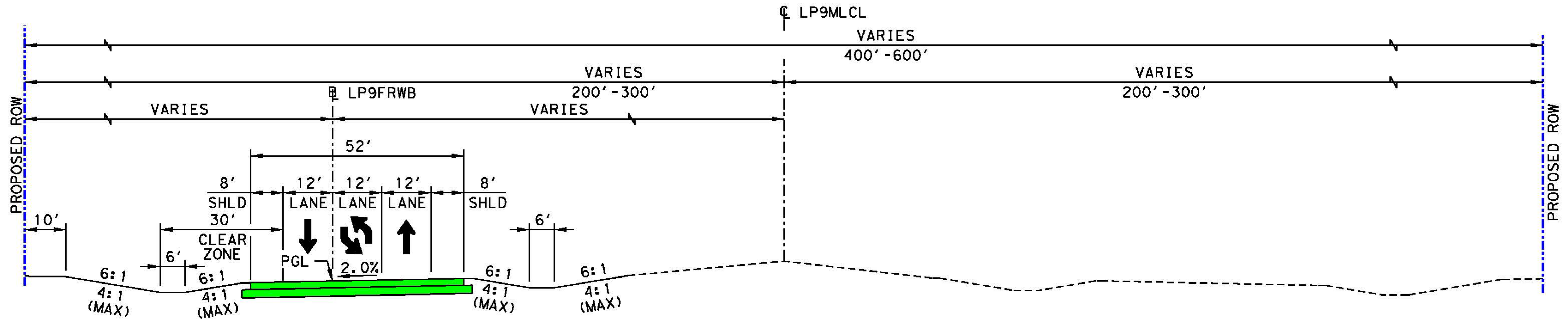
PROPOSED TYPICAL SECTION - PHASE 1 LOOP 9 - SEGMENT A
