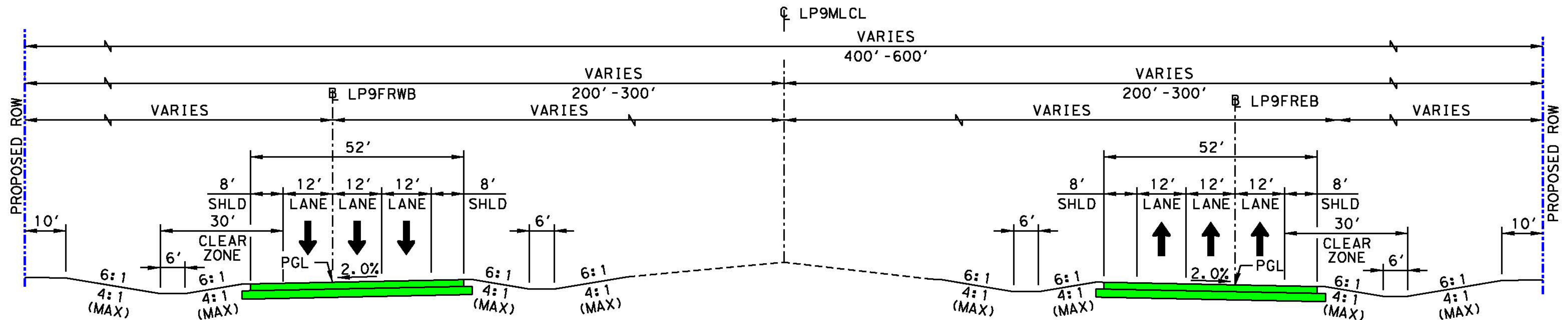
PROPOSED TYPICAL SECTION - PHASE 2 LOOP 9 - SEGMENT A
