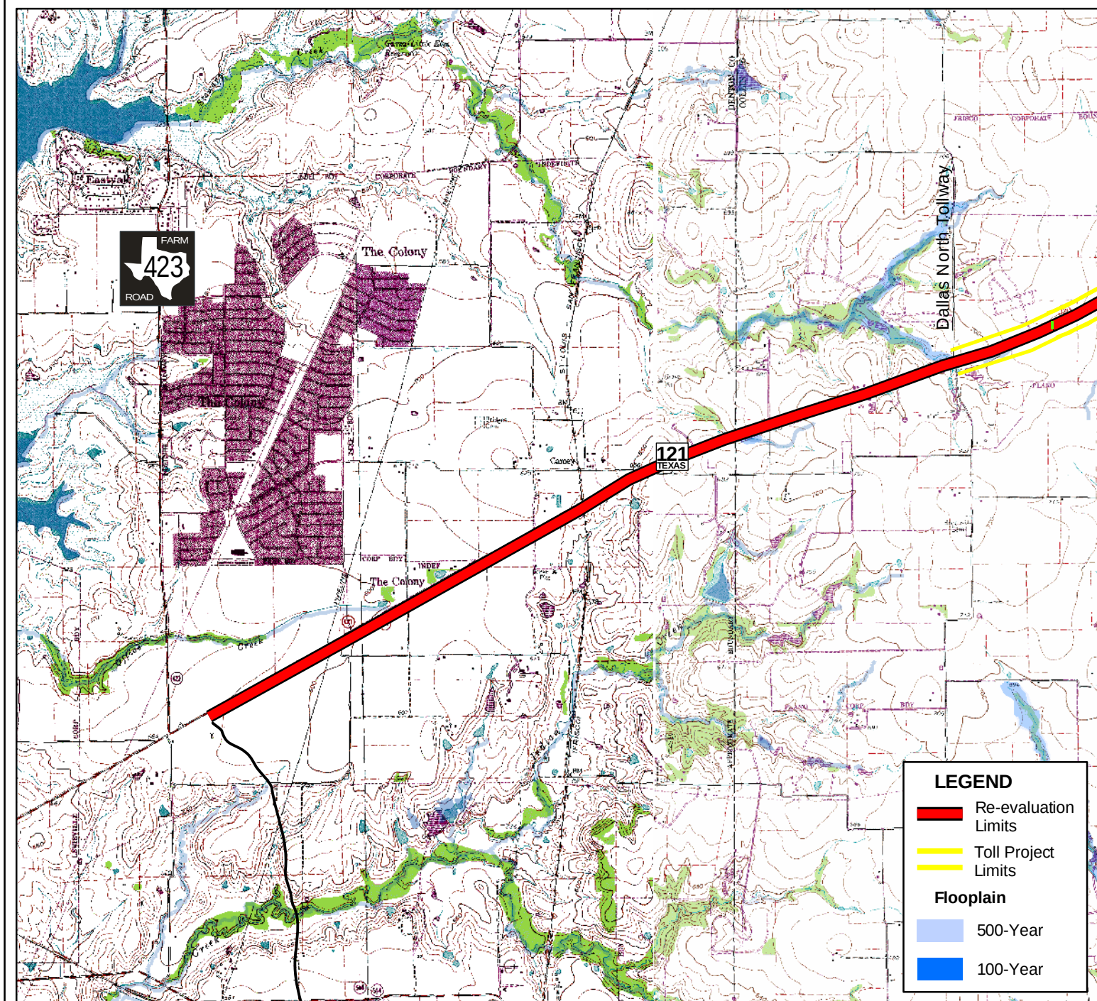
FIGURE 2 : SHEET 1 OF 3 USGS QUADRANGLE MAP AND FEMA FLOODPLAIN MAP
