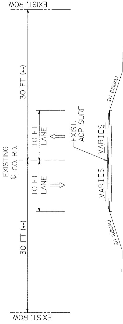
TYPICAL EXISTING ROADWAY SECTION (AT BRIDGE APPROACH)
