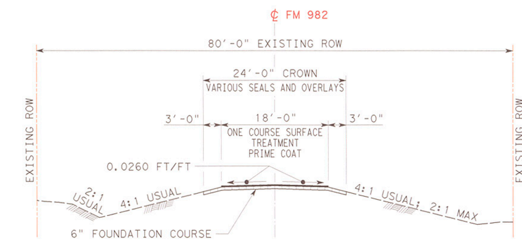
EXISTING TYPICAL SECTION NTS
