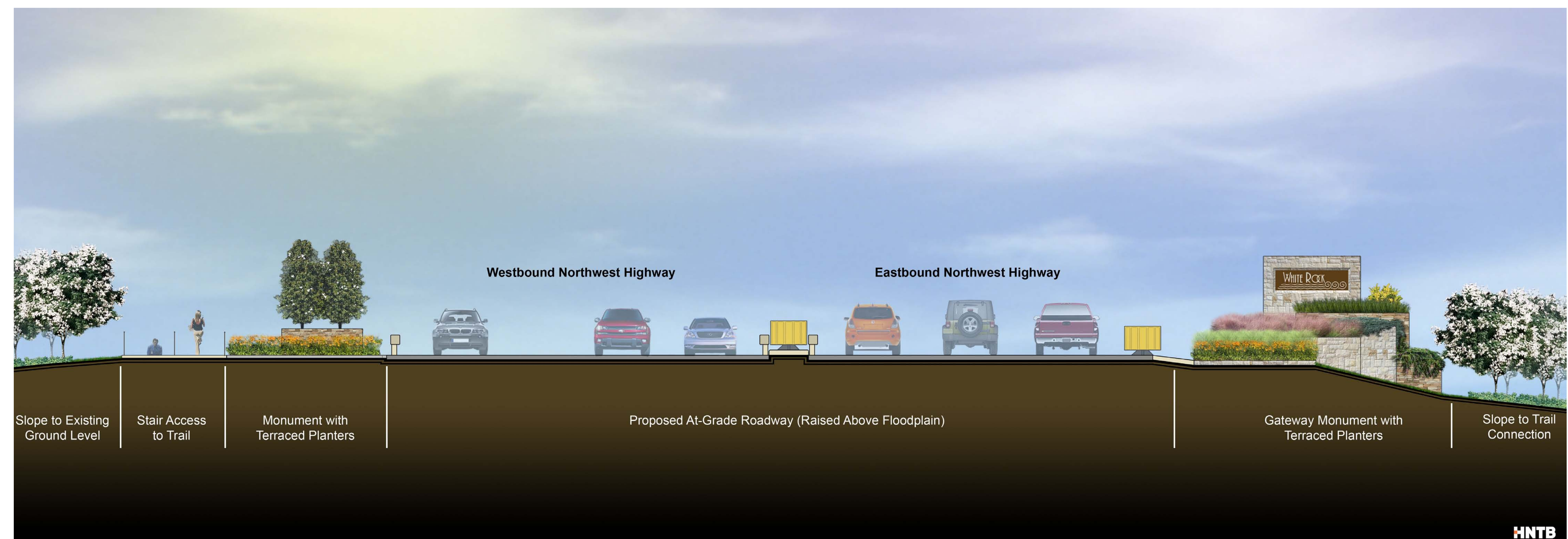
Section and Elevation Illustrations
